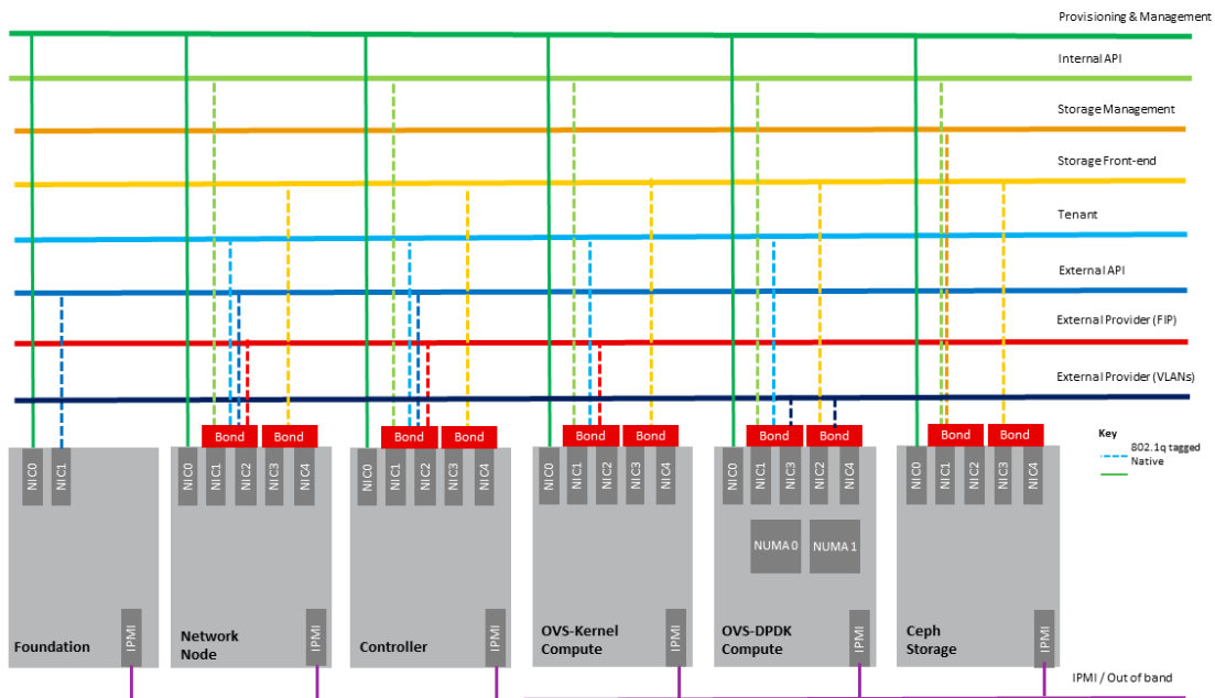
Figure 2.8: Indicative OpenStack Network Layout
