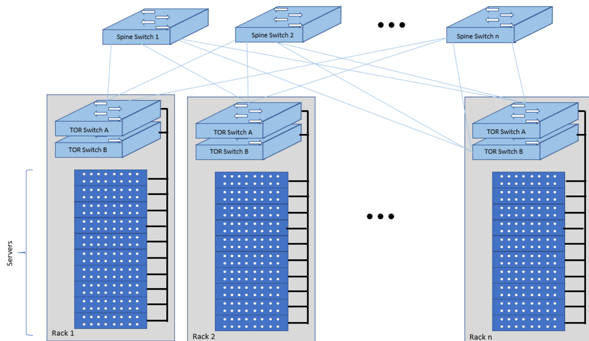
Figure 2.3: Network Fabric – Physical
