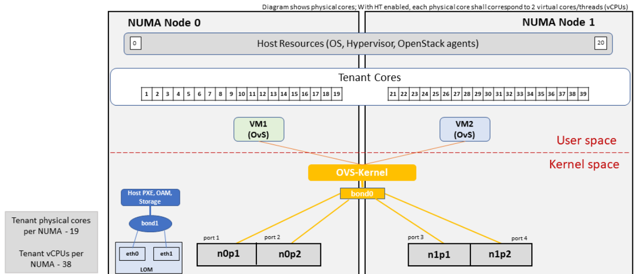
Figure 2.4: Basic Profile Host Configuration (example and simplified)
