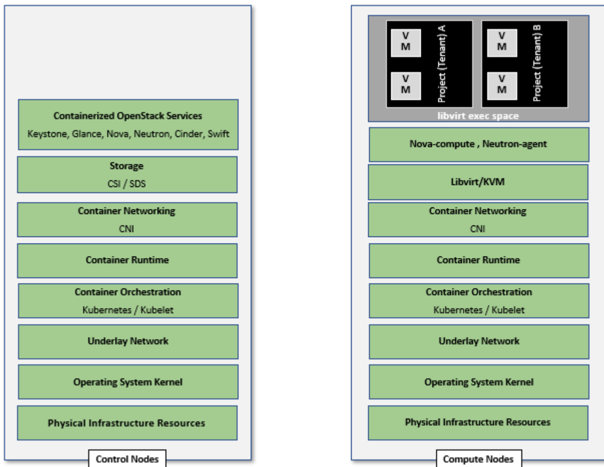
Figure 2.10: Containerised OpenStack Services Topology
