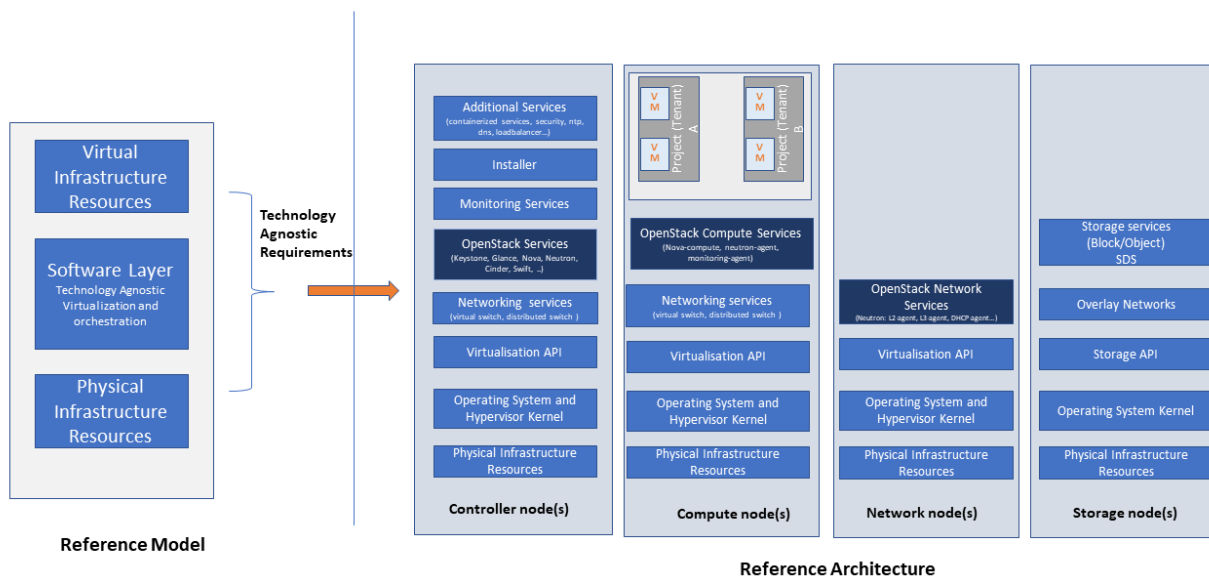
Figure 2.2: OpenStack Services Topology
