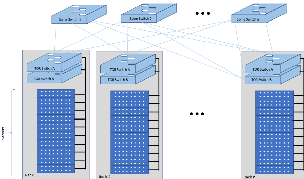
Fig. 3.3: Network Fabric – Physical
